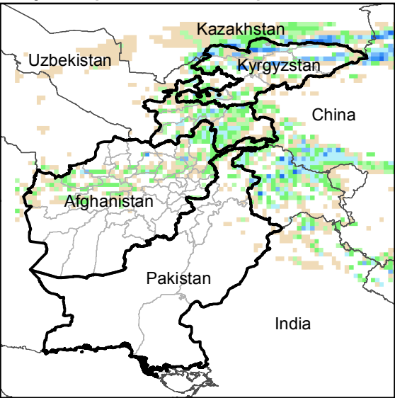
Daily Precip. Forecast for 4 Apr., 2017
