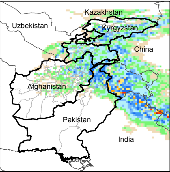
Daily Precip. Forecast for 5 Apr., 2017
