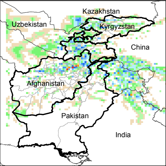
Daily Precip. Forecast for 20 Apr., 2017
