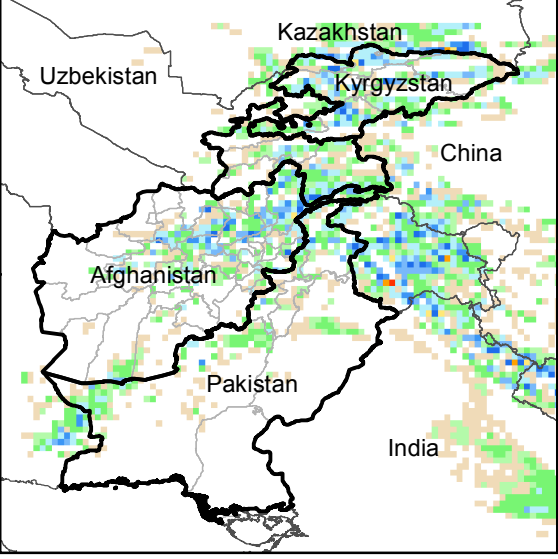
Daily Precip. Forecast for 21 Apr., 2017
