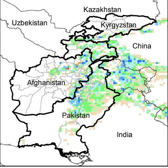
Daily Precip. Forecast for 23 Apr., 2017
