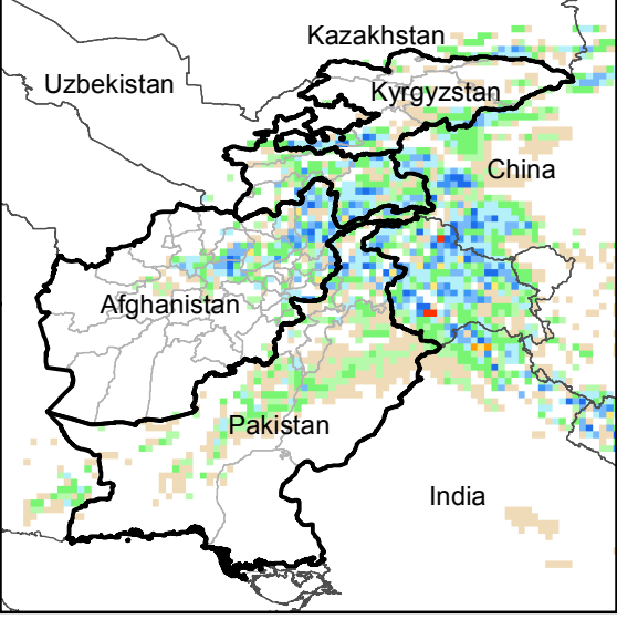
Daily Precip. Forecast for 22 Apr., 2017
