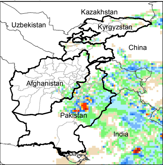
Daily Precip. Forecast for 10 Jun., 2017
