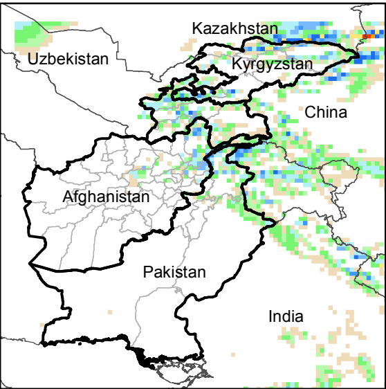
Daily Precip. Forecast for 8 Jun., 2017
