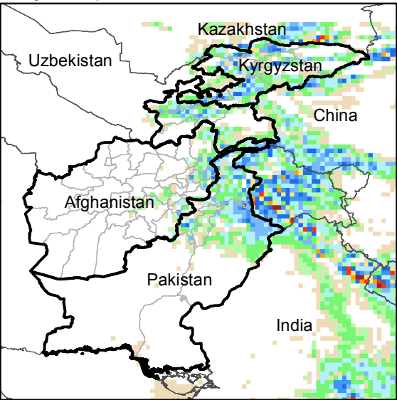
Daily Precip. Forecast for 9 Jun., 2017
