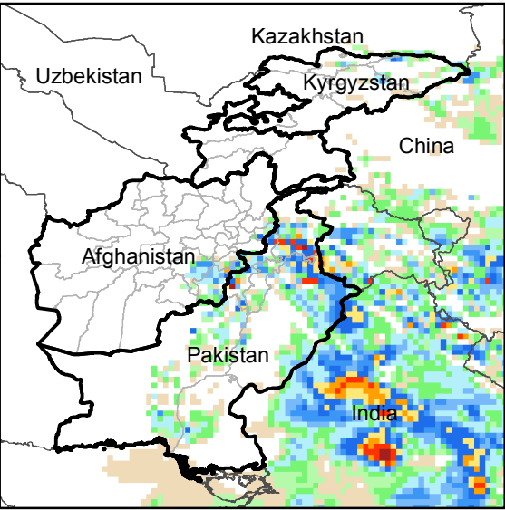
Daily Precip. Forecast for 30 Jul., 2017
