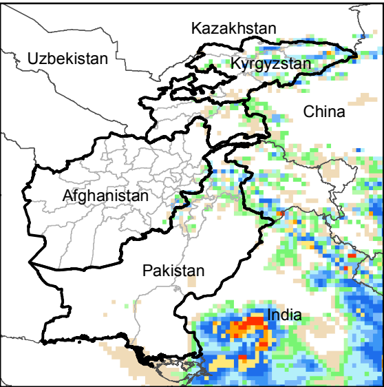
Daily Precip. Forecast for 28 Jul., 2017
