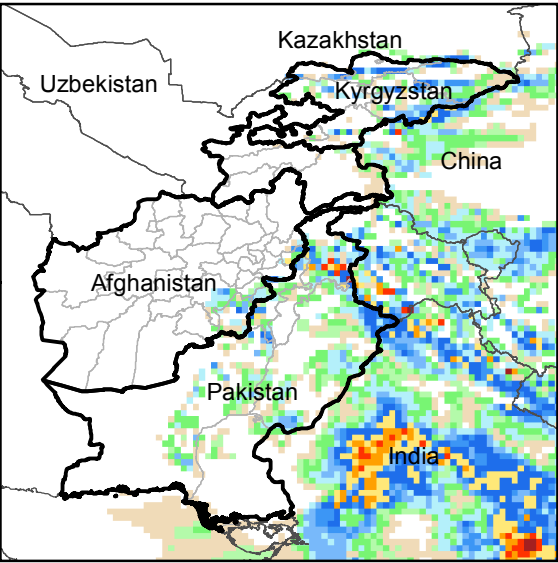
Daily Precip. Forecast for 29 Jul., 2017
