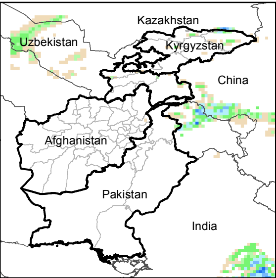
Daily Precip. Forecast for 16 Oct., 2017
