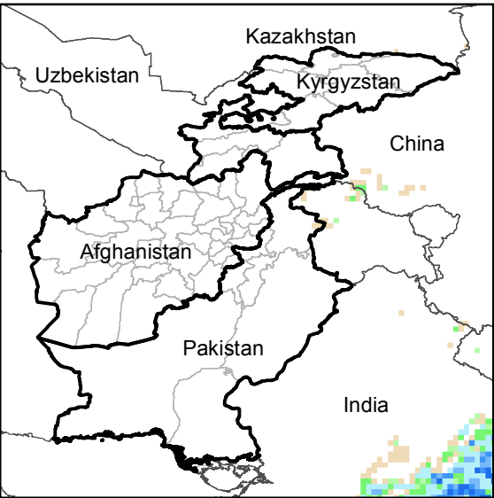
Daily Precip. Forecast for 23 Oct., 2017
