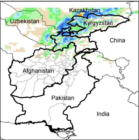
Daily Precip. Forecast for 29 Nov., 2017
