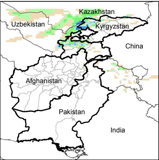
Daily Precip. Forecast for 2 Dec., 2017
