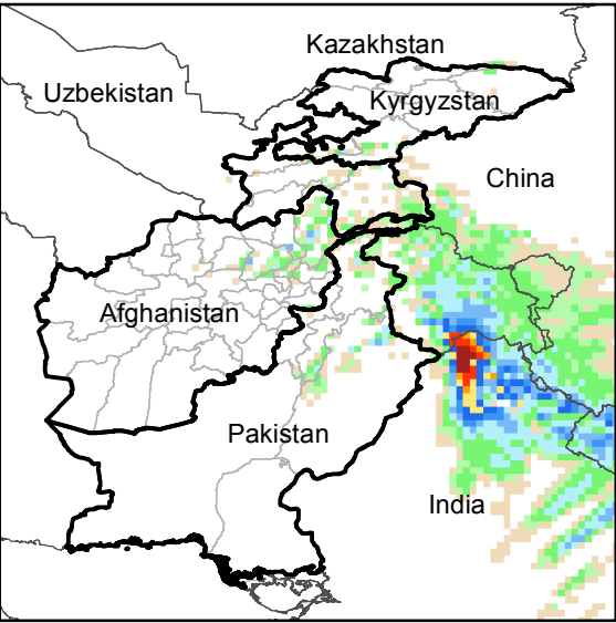
Daily Precip. Forecast for 12 Dec., 2017
