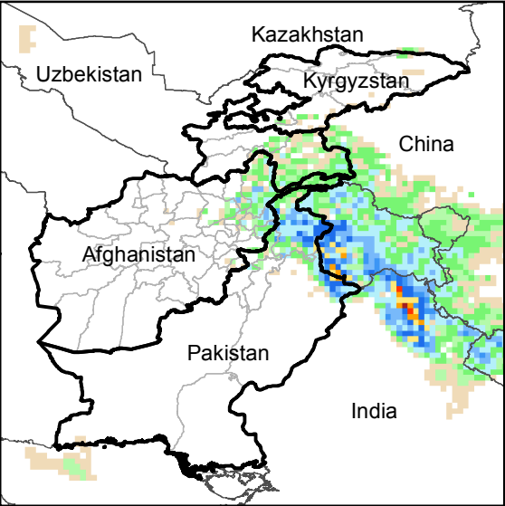
Daily Precip. Forecast for 15 Dec., 2017
