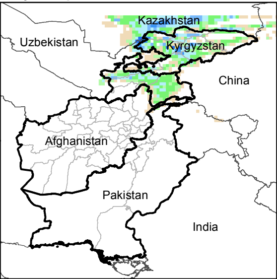
Daily Precip. Forecast for 16 Jan., 2018
