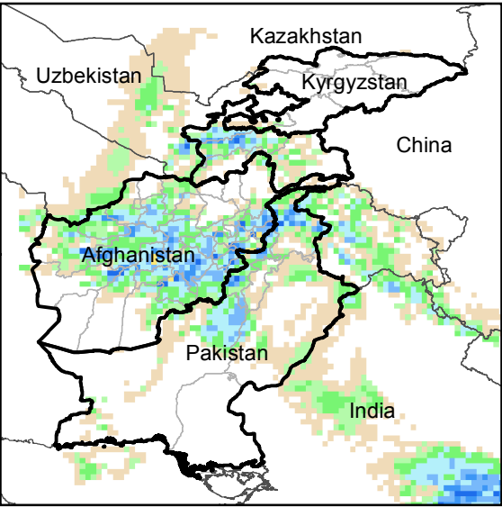
Daily Precip. Forecast for 11 Feb., 2018
