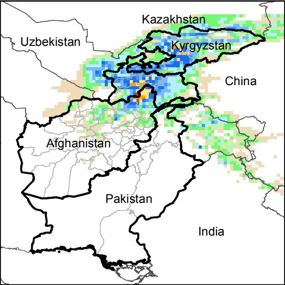
Daily Precip. Forecast for 18 Feb., 2018
