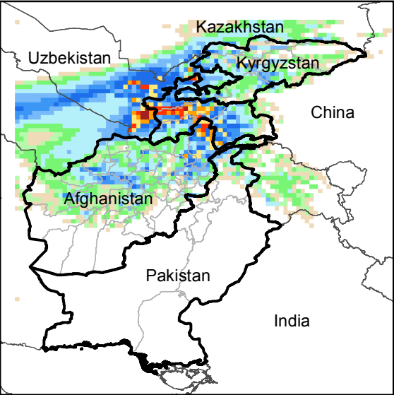
Daily Precip. Forecast for 17 Feb., 2018
