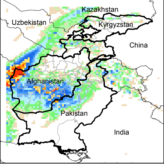
Daily Precip. Forecast for 25 Feb., 2018
