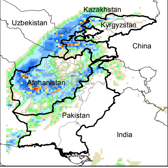
Daily Precip. Forecast for 26 Feb., 2018
