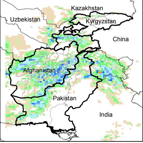
Daily Precip. Forecast for 24 Feb., 2018
