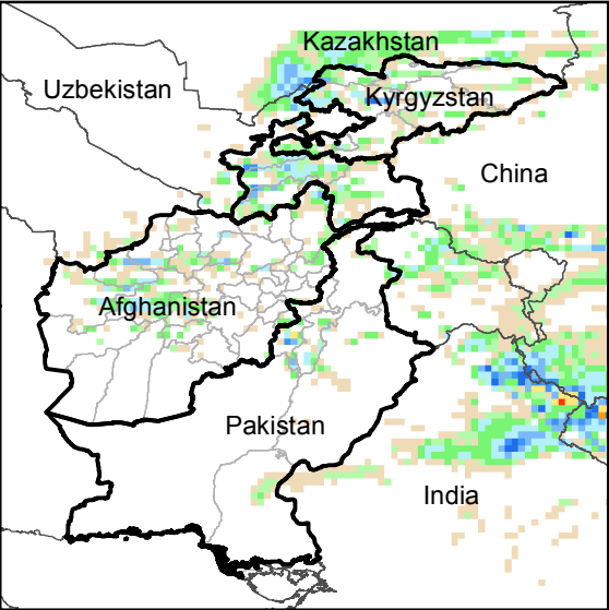
Daily Precip. Forecast for 4 Mar., 2018
