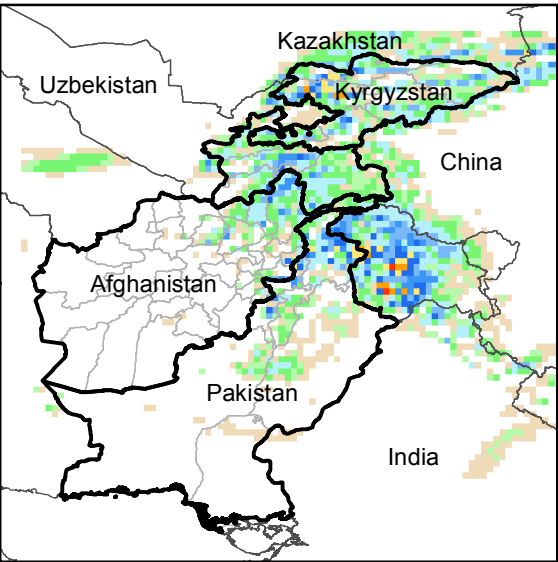
Daily Precip. Forecast for 17 Mar., 2018
