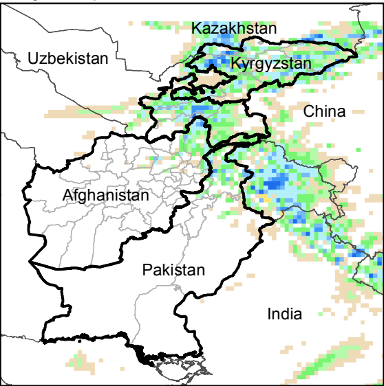
Daily Precip. Forecast for 18 Mar., 2018
