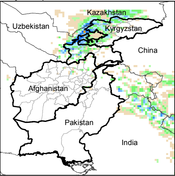
Daily Precip. Forecast for 22 Mar., 2018
