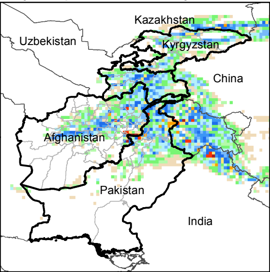
Daily Precip. Forecast for 9 May., 2018
