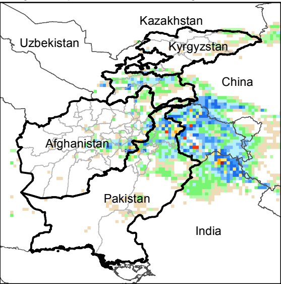
Daily Precip. Forecast for 10 May., 2018
