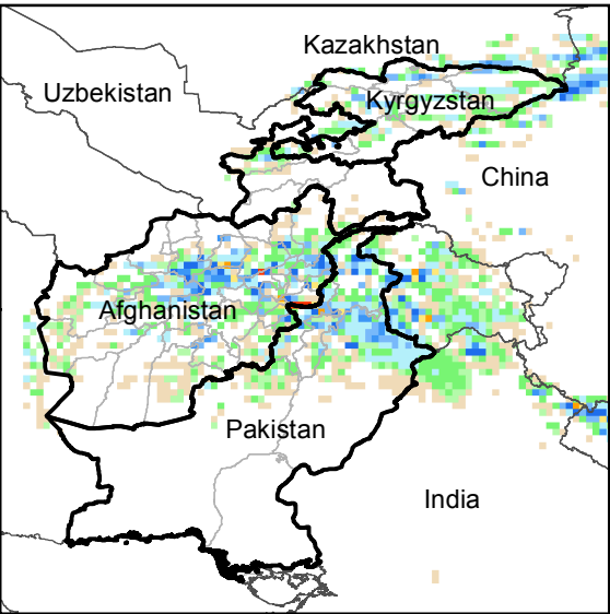
Daily Precip. Forecast for 8 May., 2018
