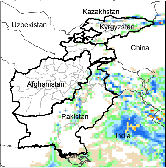
Daily Precip. Forecast for 9 Aug., 2018
