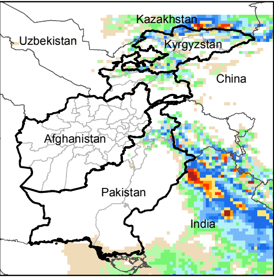
Daily Precip. Forecast for 11 Aug., 2018
