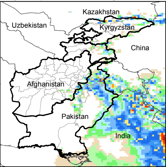
Daily Precip. Forecast for 10 Aug., 2018
