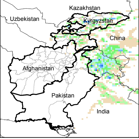
Daily Precip. Forecast for 14 Nov., 2018
