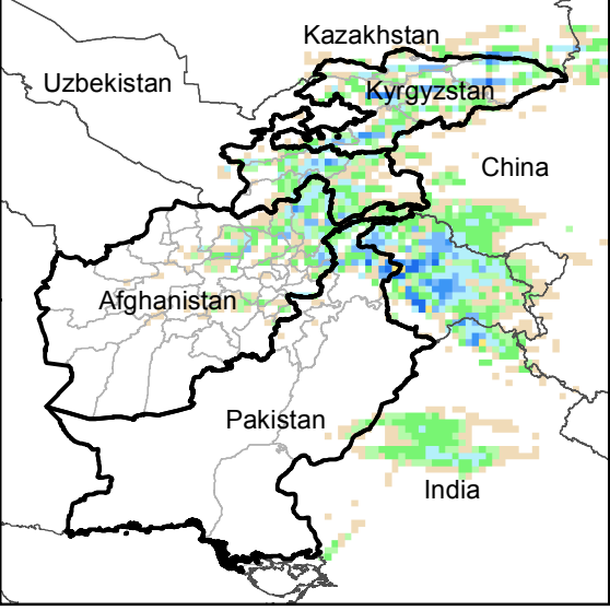
Daily Precip. Forecast for 13 Nov., 2018
