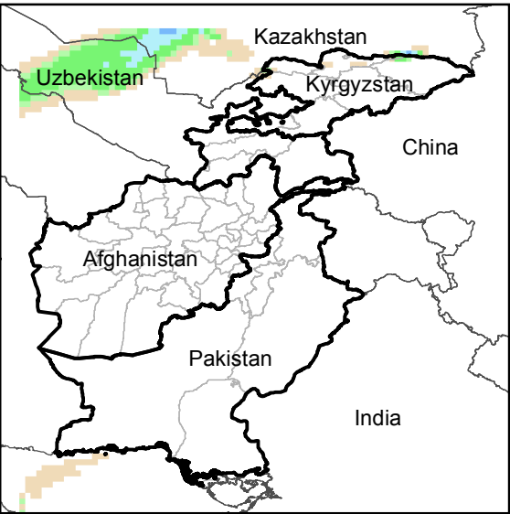
Daily Precip. Forecast for 18 Dec., 2018
