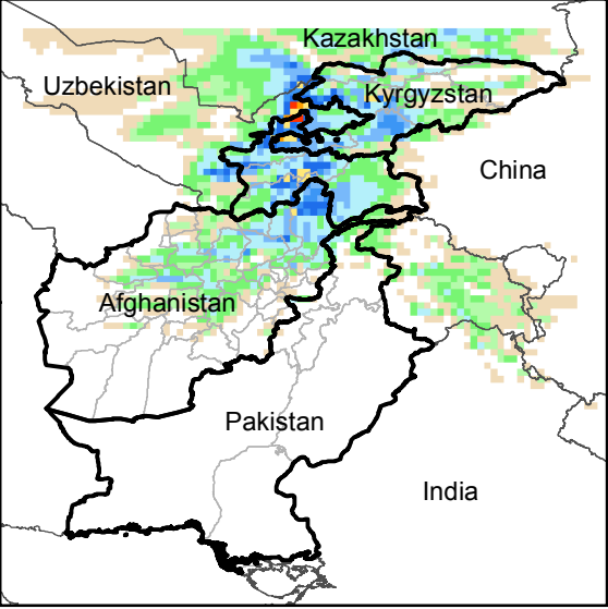
Daily Precip. Forecast for 8 Jan., 2019
