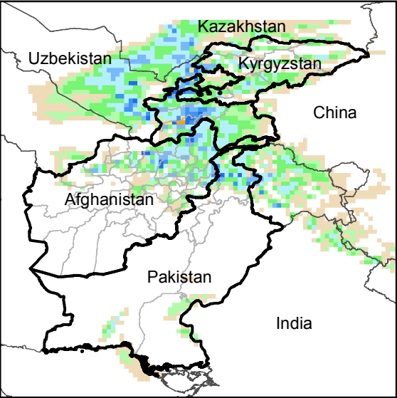
Daily Precip. Forecast for 14 Jan., 2019
