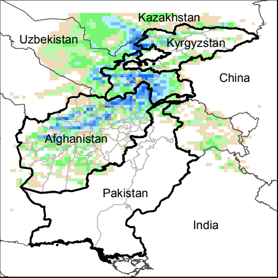
Daily Precip. Forecast for 15 Jan., 2019
