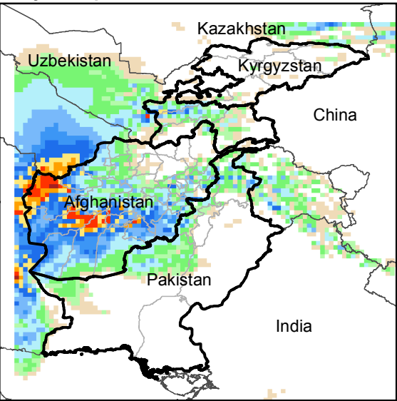
Daily Precip. Forecast for 15 Feb., 2019
