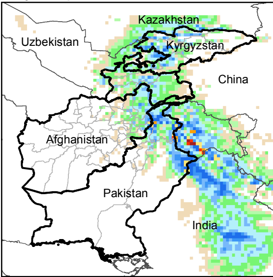
Daily Precip. Forecast for 17 Feb., 2019
