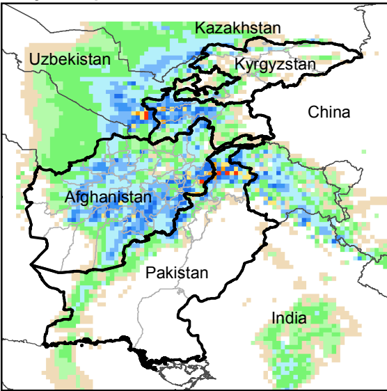
Daily Precip. Forecast for 16 Feb., 2019
