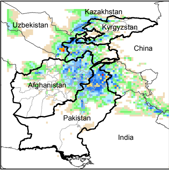
Daily Precip. Forecast for 19 Mar., 2019
