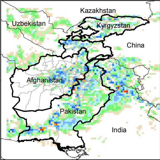
Daily Precip. Forecast for 19 May., 2019
