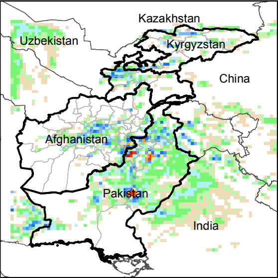
Daily Precip. Forecast for 18 May., 2019
