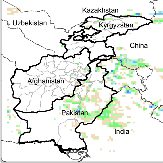
Daily Precip. Forecast for 20 May., 2019
