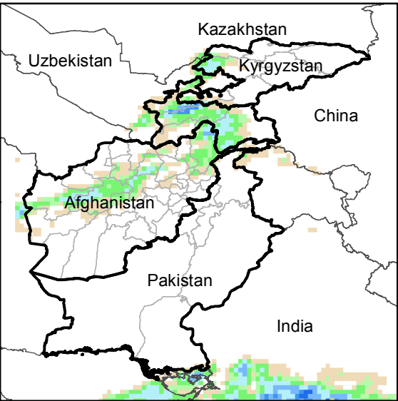
Daily Precip. Forecast for 30 Oct., 2019
