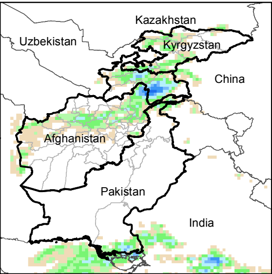
Daily Precip. Forecast for 31 Oct., 2019
