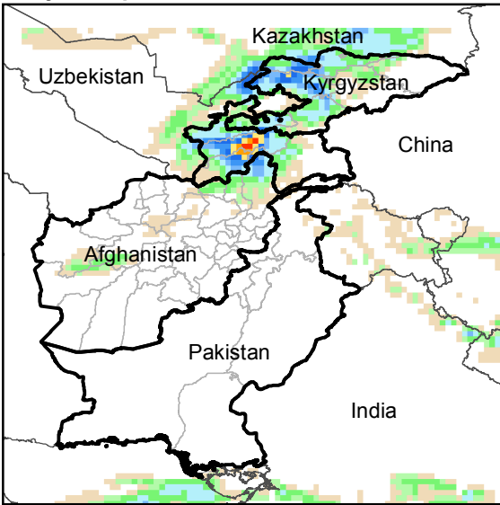
Daily Precip. Forecast for 7 Nov., 2019
