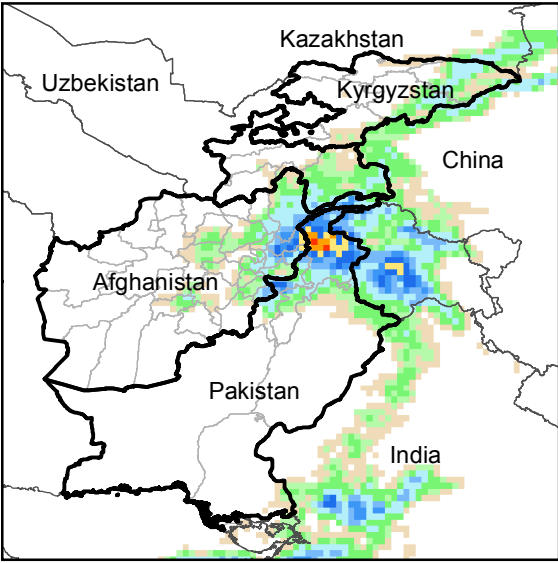
Daily Precip. Forecast for 6 Nov., 2019
