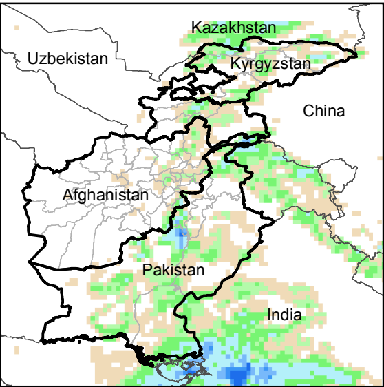
Daily Precip. Forecast for 5 Nov., 2019
