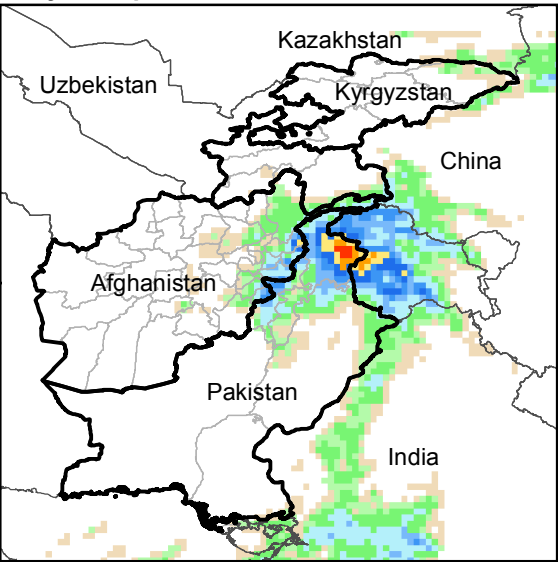
Daily Precip. Forecast for 9 Nov., 2019
