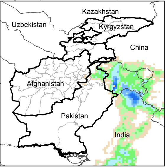
Daily Precip. Forecast for 8 Nov., 2019
