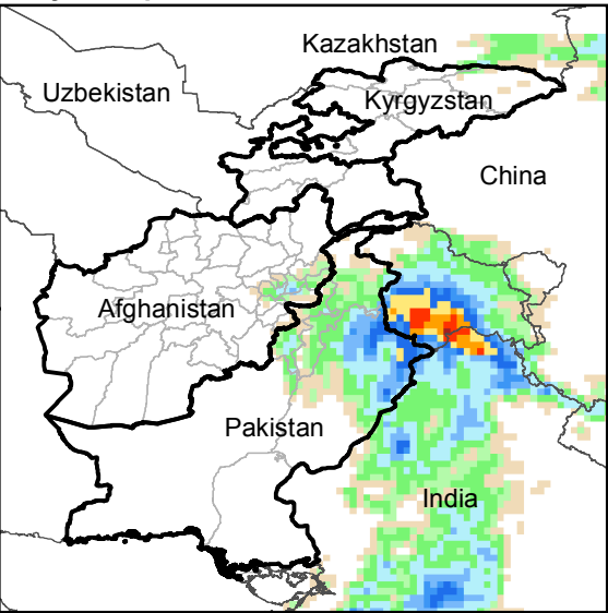
Daily Precip. Forecast for 10 Nov., 2019
