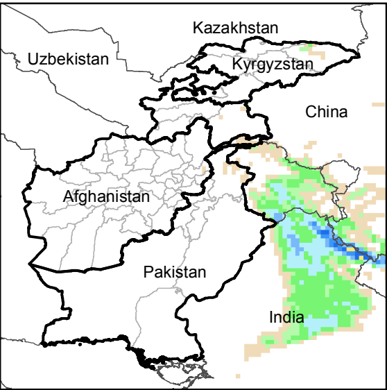
Daily Precip. Forecast for 1 Dec., 2019
