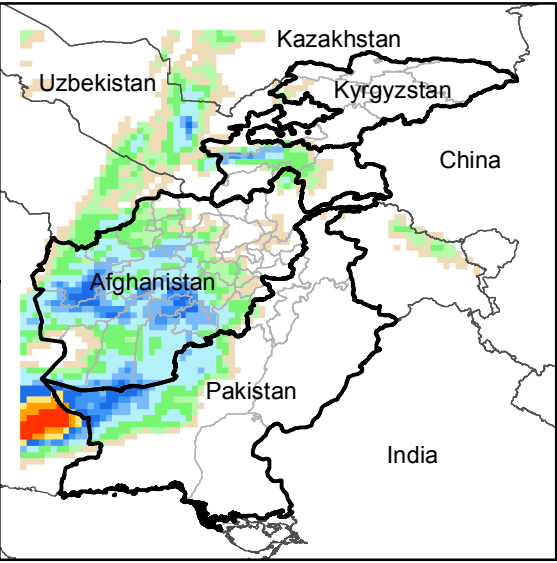
Daily Precip. Forecast for 10 Dec., 2019
