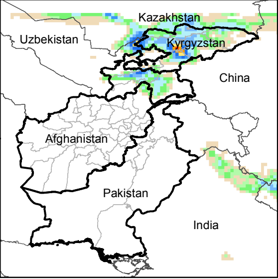
Daily Precip. Forecast for 21 Dec., 2019
