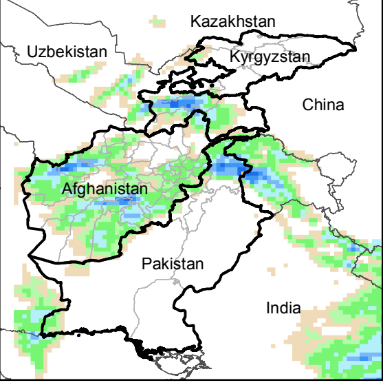
Daily Precip. Forecast for 2 Jan., 2020
