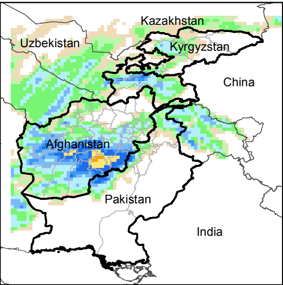
Daily Precip. Forecast for 14 Feb., 2020
