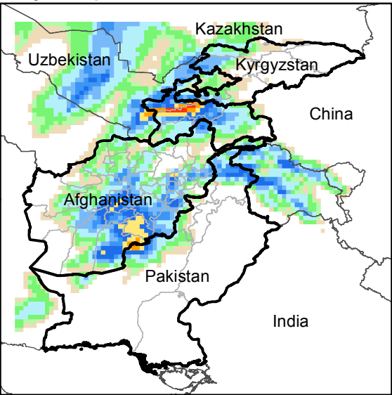
Daily Precip. Forecast for 15 Feb., 2020
