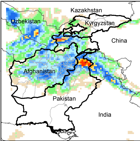
Daily Precip. Forecast for 3 Apr., 2020
