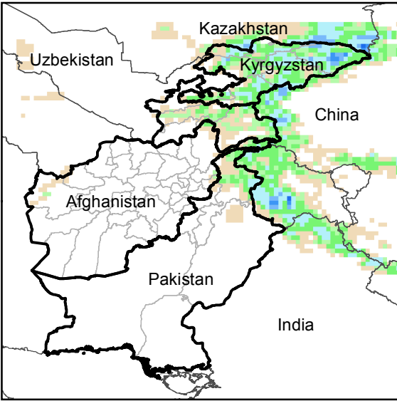
Daily Precip. Forecast for 2 Apr., 2020
