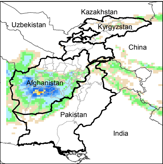
Daily Precip. Forecast for 1 Apr., 2020
