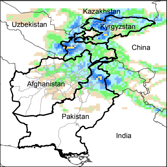
Daily Precip. Forecast for 4 Apr., 2020
