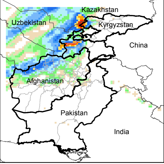
Daily Precip. Forecast for 12 Apr., 2020
