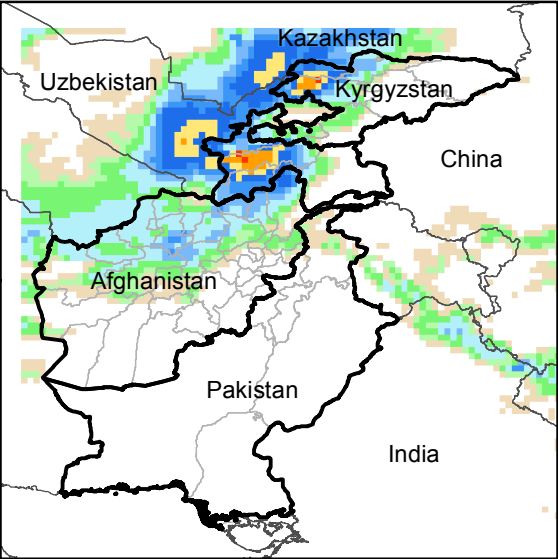
Daily Precip. Forecast for 8 Apr., 2020
