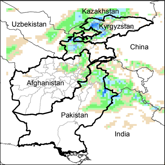
Daily Precip. Forecast for 7 Apr., 2020
