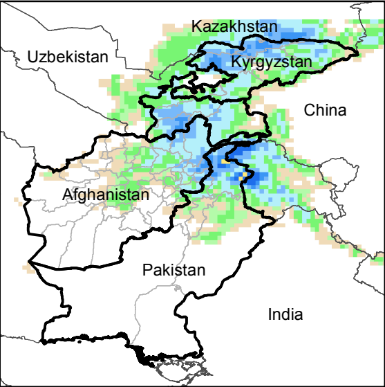
Daily Precip. Forecast for 9 Apr., 2020
