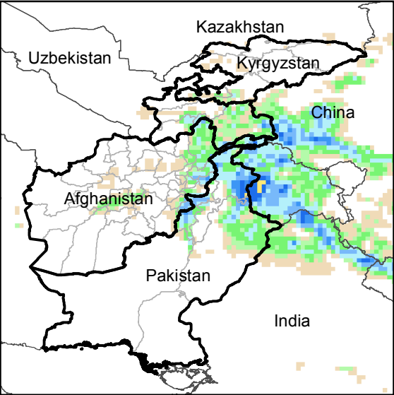
Daily Precip. Forecast for 18 Apr., 2020
