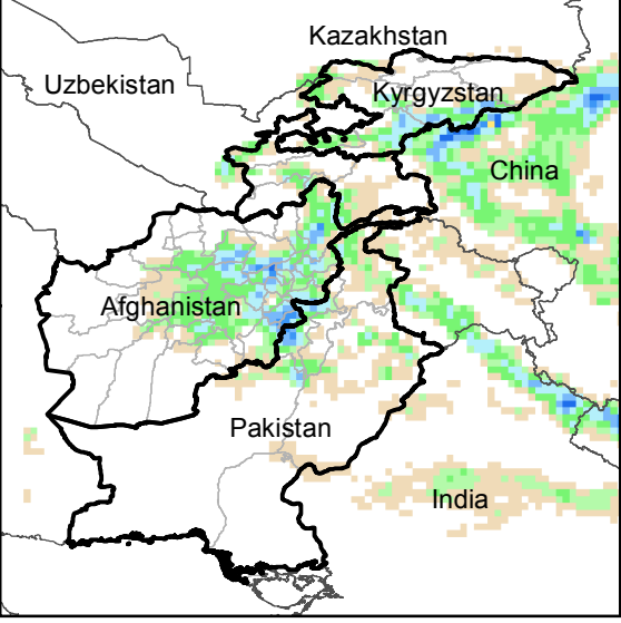
Daily Precip. Forecast for 20 Apr., 2020
