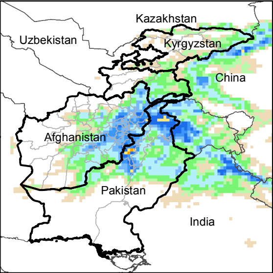
Daily Precip. Forecast for 17 Apr., 2020
