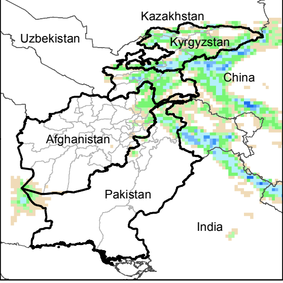
Daily Precip. Forecast for 21 Apr., 2020
