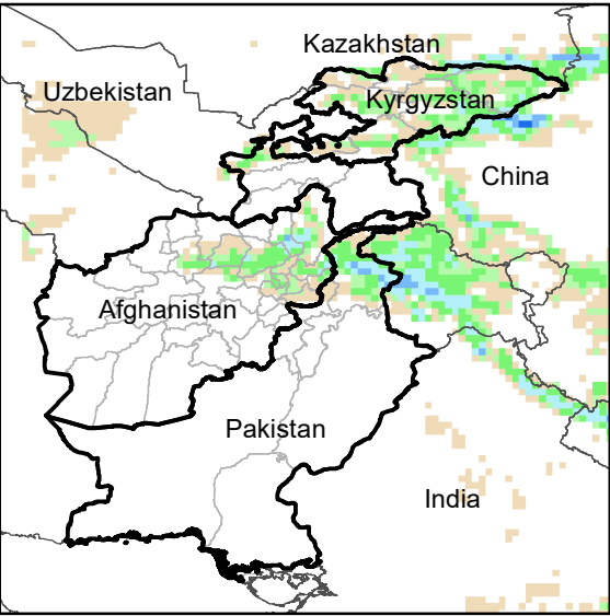
Daily Precip. Forecast for 10 May., 2020
