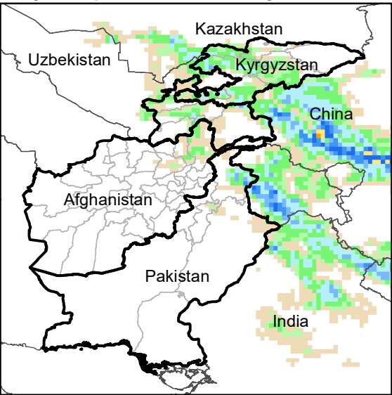
Daily Precip. Forecast for 9 May., 2020
