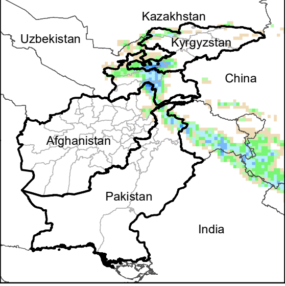
Daily Precip. Forecast for 26 May., 2020
