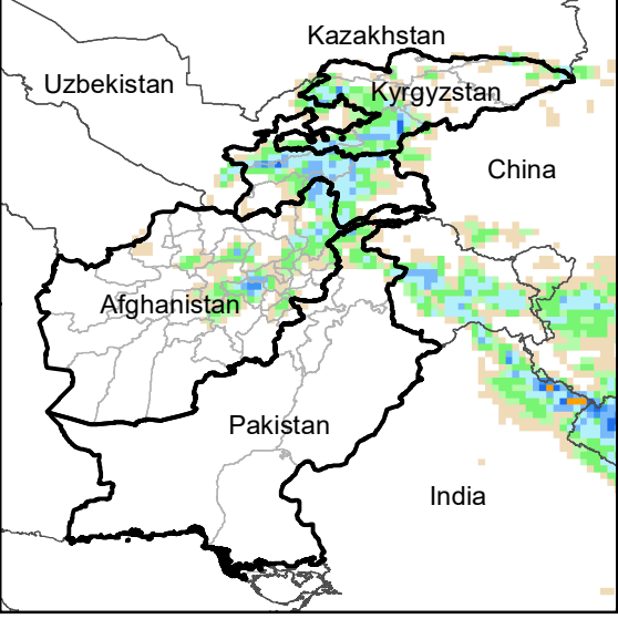
Daily Precip. Forecast for 28 May., 2020
