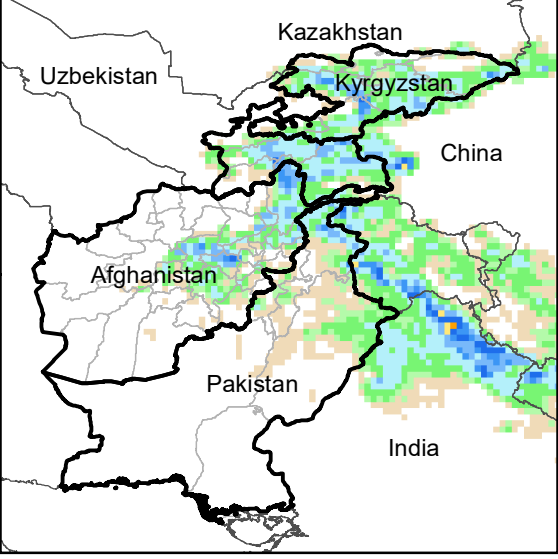
Daily Precip. Forecast for 29 May., 2020
