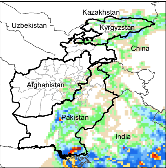
Daily Precip. Forecast for 9 Jul., 2020
