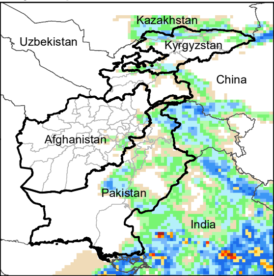
Daily Precip. Forecast for 8 Jul., 2020
