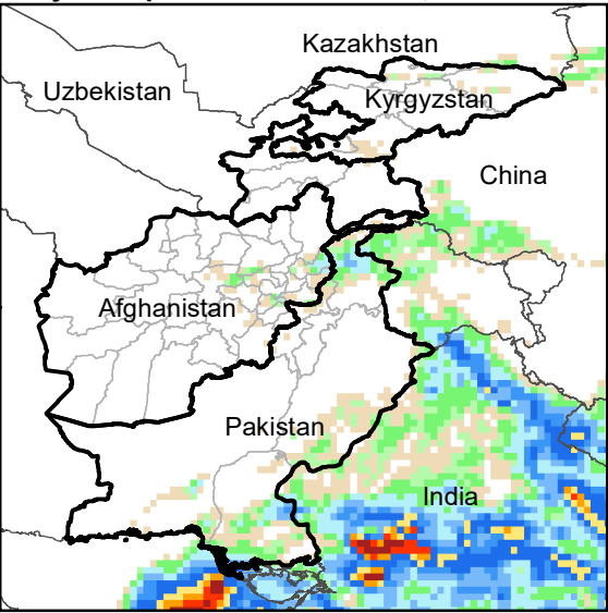
Daily Precip. Forecast for 7 Jul., 2020
