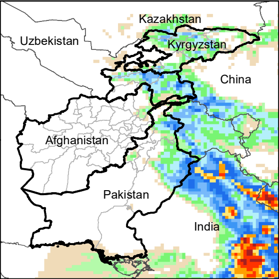
Daily Precip. Forecast for 20 Jul., 2020
