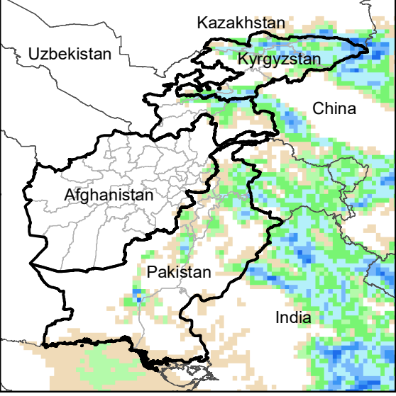
Daily Precip. Forecast for 22 Jul., 2020
