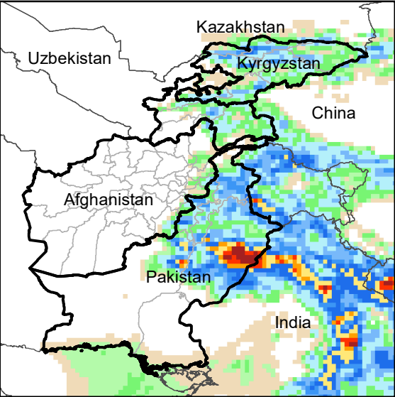
Daily Precip. Forecast for 21 Jul., 2020
