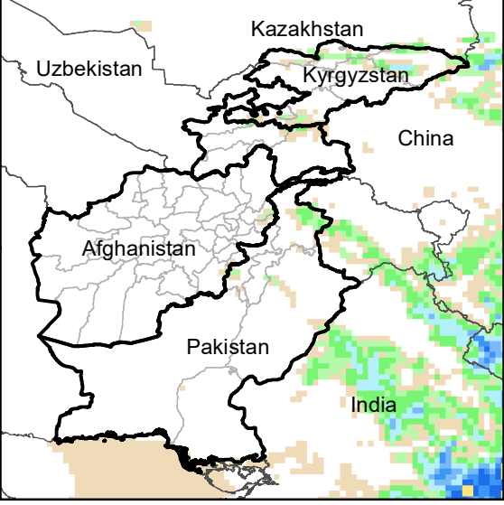
Daily Precip. Forecast for 23 Jul., 2020
