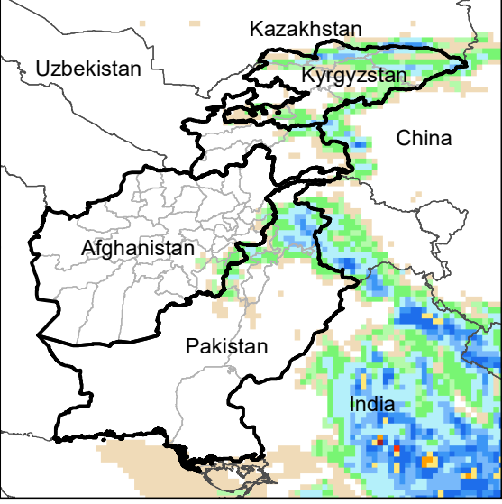
Daily Precip. Forecast for 24 Jul., 2020
