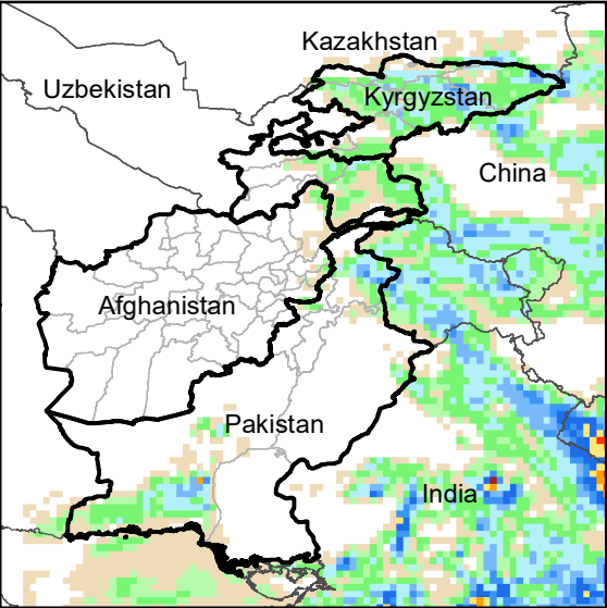
Daily Precip. Forecast for 19 Jul., 2020
