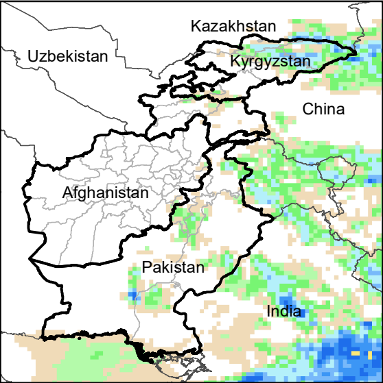
Daily Precip. Forecast for 25 Jul., 2020
