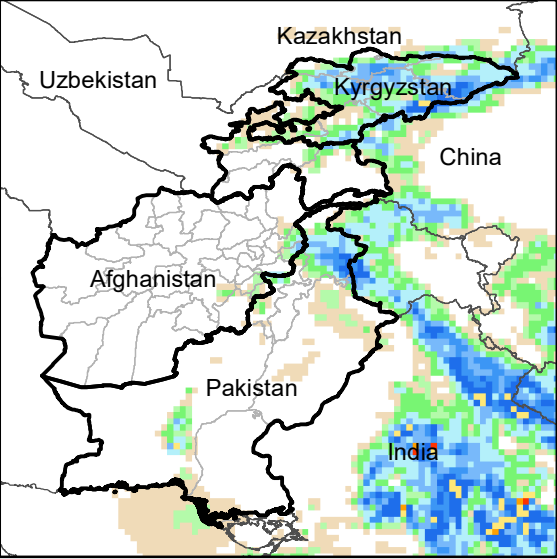
Daily Precip. Forecast for 26 Jul., 2020
