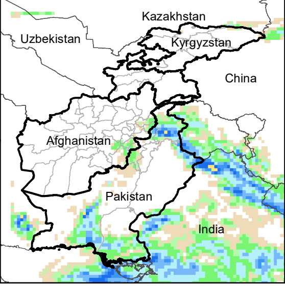
Daily Precip. Forecast for 25 Aug., 2020
