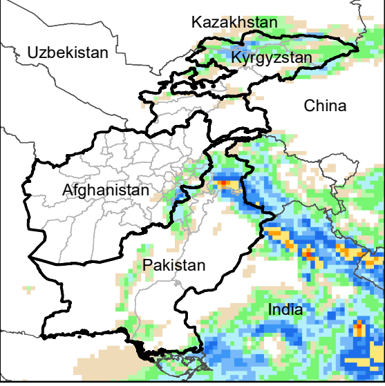
Daily Precip. Forecast for 26 Aug., 2020
