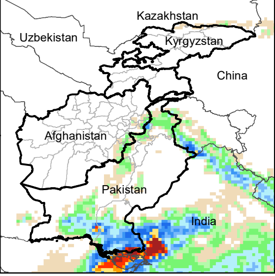
Daily Precip. Forecast for 24 Aug., 2020
