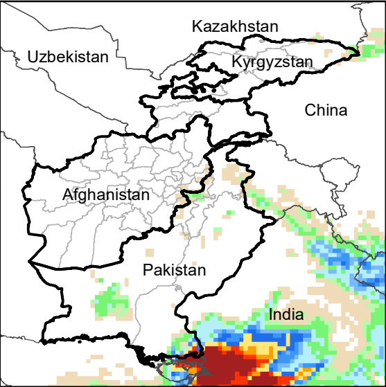
Daily Precip. Forecast for 23 Aug., 2020
