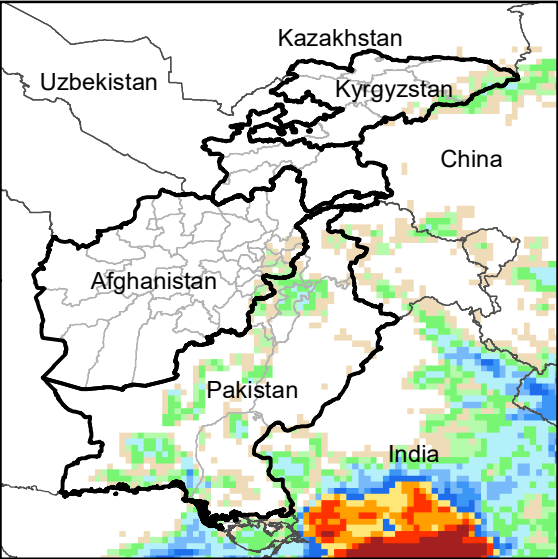
Daily Precip. Forecast for 22 Aug., 2020
