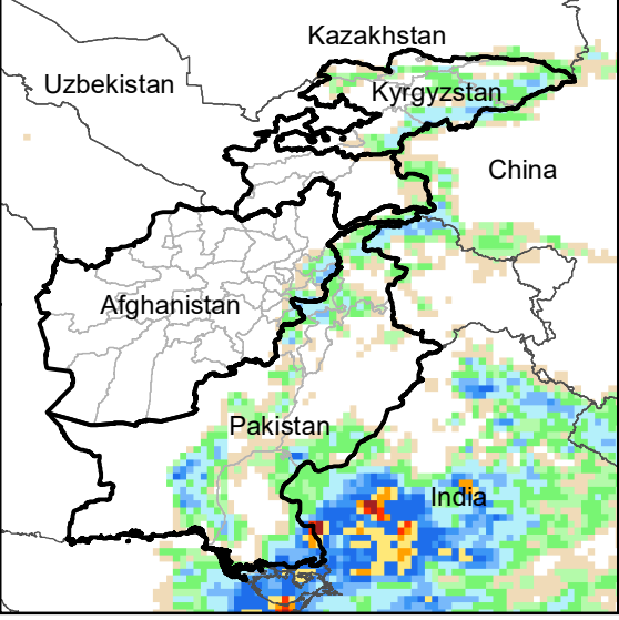
Daily Precip. Forecast for 30 Aug., 2020
