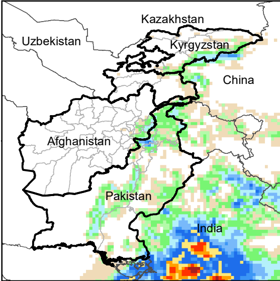
Daily Precip. Forecast for 29 Aug., 2020
