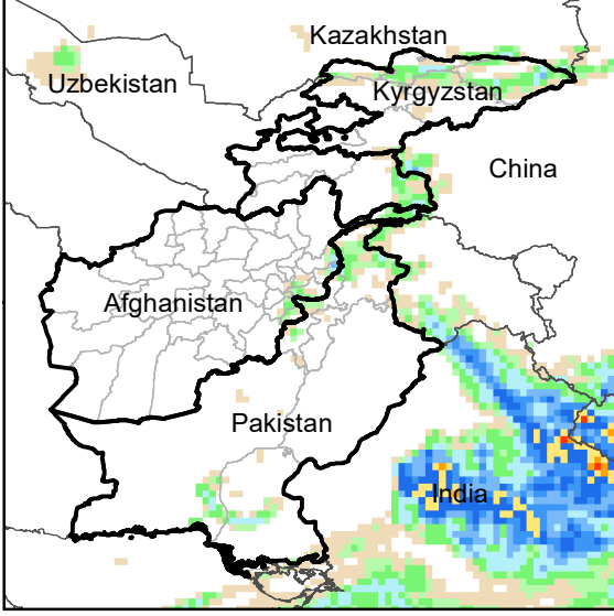
Daily Precip. Forecast for 1 Sep., 2020
