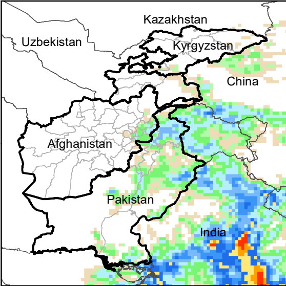
Daily Precip. Forecast for 28 Aug., 2020
