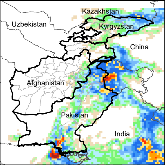
Daily Precip. Forecast for 27 Aug., 2020
