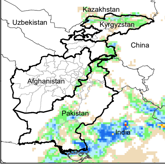
Daily Precip. Forecast for 31 Aug., 2020
