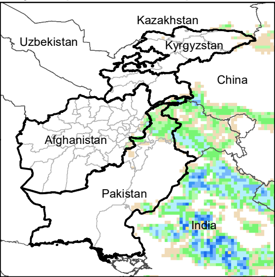
Daily Precip. Forecast for 8 Sep., 2020
