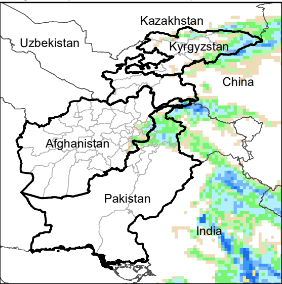
Daily Precip. Forecast for 9 Sep., 2020
