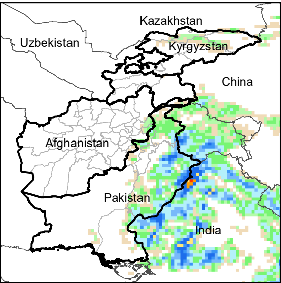
Daily Precip. Forecast for 7 Sep., 2020
