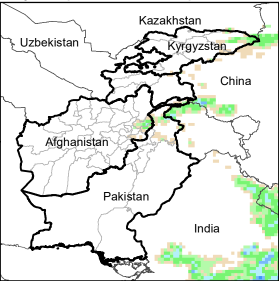
Daily Precip. Forecast for 12 Sep., 2020
